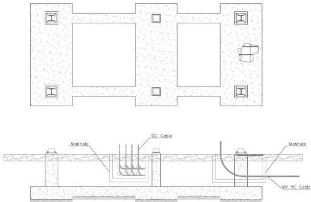
Figure 14 – ITC foundation example
