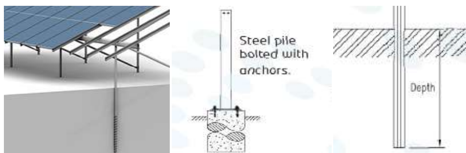
Figure 12 – Krinner screw, reinforced concrete foundation and drive steel profile
