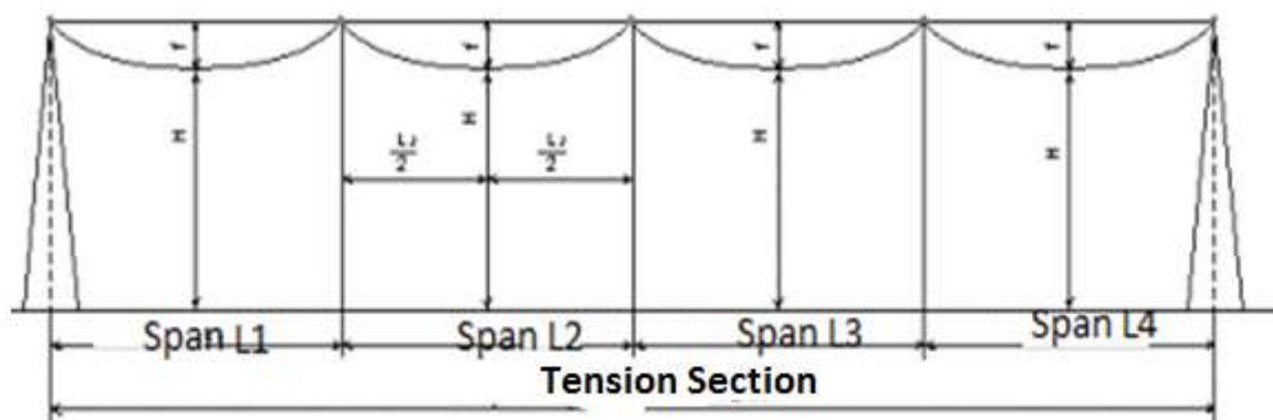
Figure 3 – Scheme of 10 kV overhead lines
