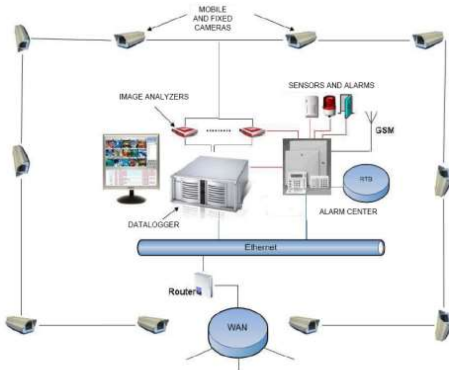
Figure 5 – Security Schema
