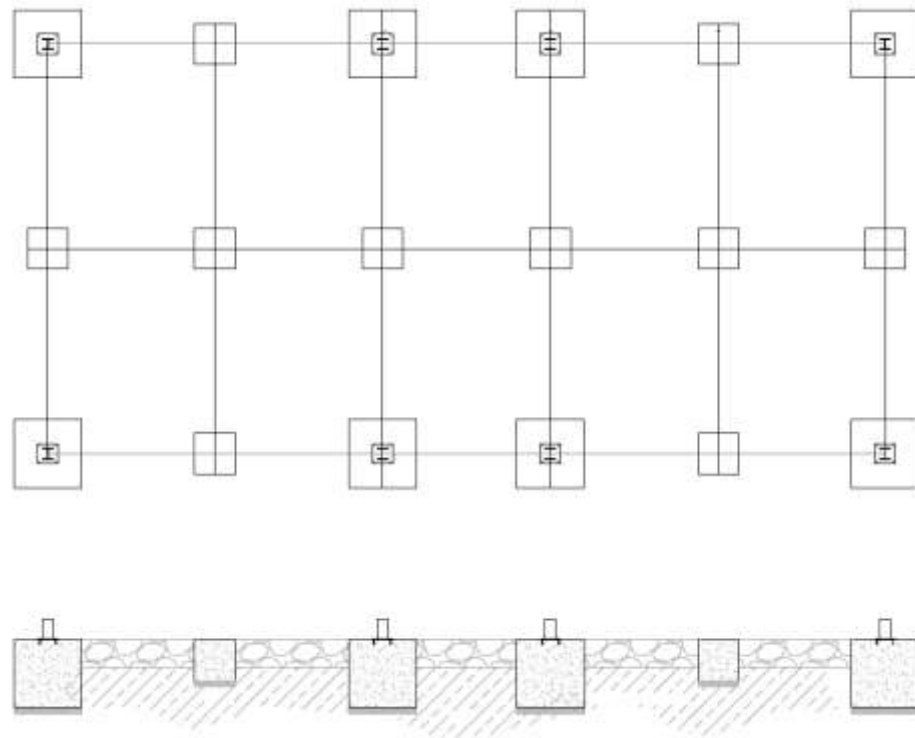
Figure 15 – Control Center and Warehouse foundation example
