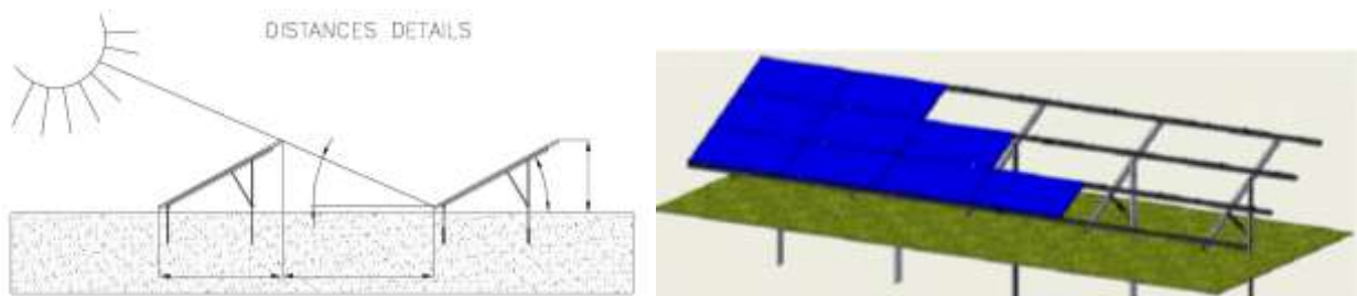
Figure 11 – Views of the PV structure
