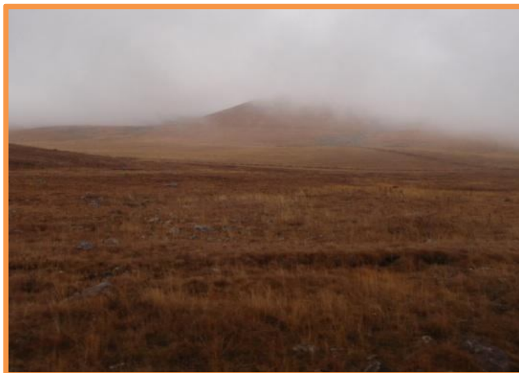
Figure 3-13. Typical Autumn Alpine Habitat of the area
