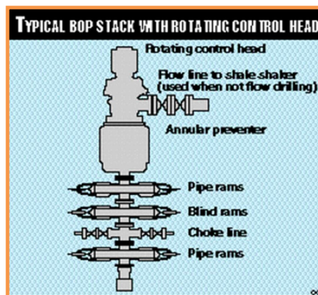
Figure 4-1. Blowout Preventer
