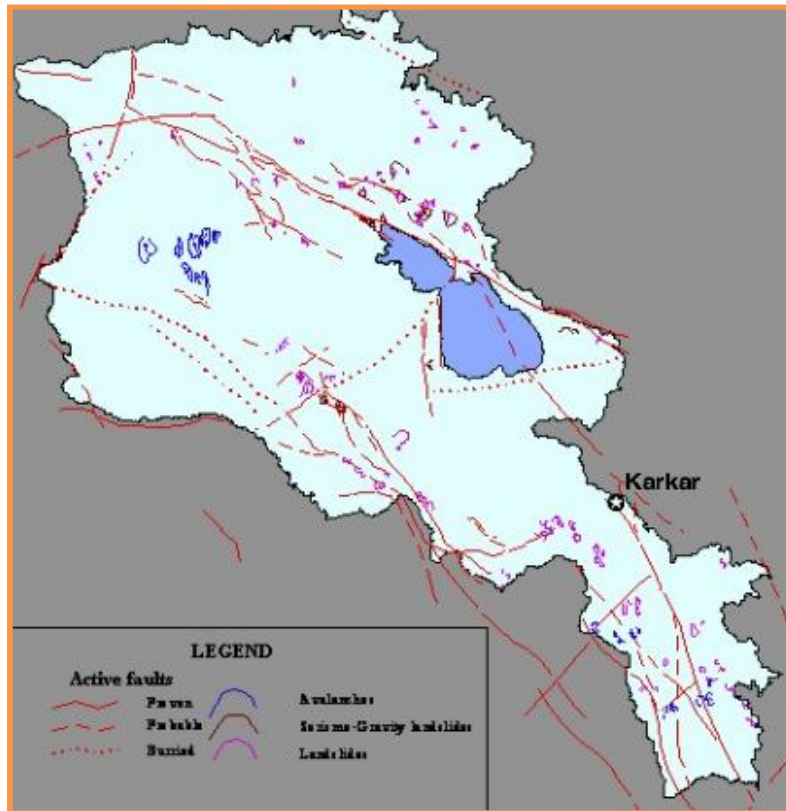
Figure 3-7. Map of Geological Fault Zones in Armenia
