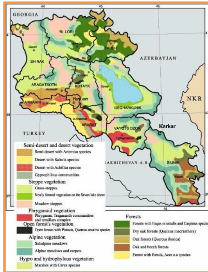
Figure 3-12. Vegetation and Habitat Zones of Armenia
